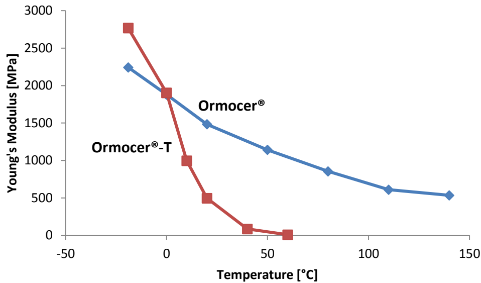
Figure 1: Young's modulus as a function of temperature for Ormocer® and Ormocer®-T.
