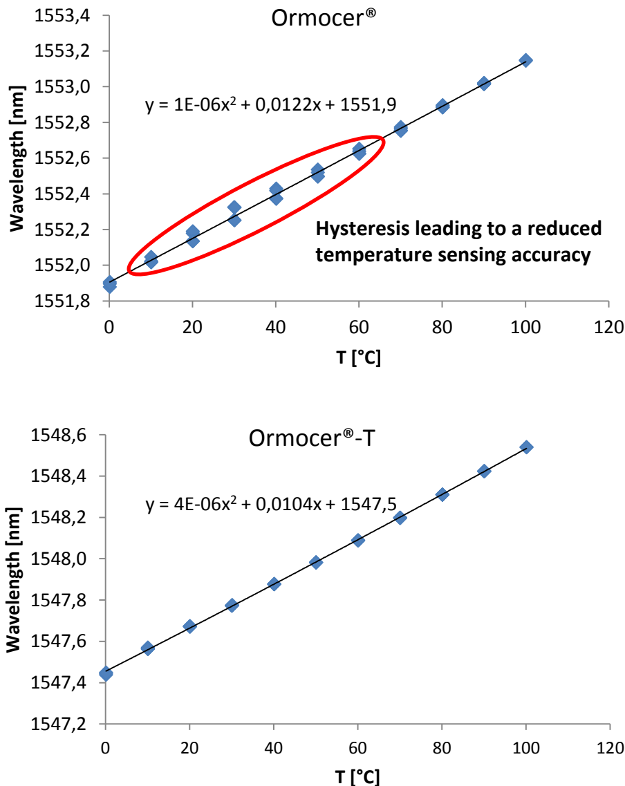
Figure 4: Temperature calibration curves for Ormocer ® (top) and Ormocer ® -T (bottom) coated samples.
