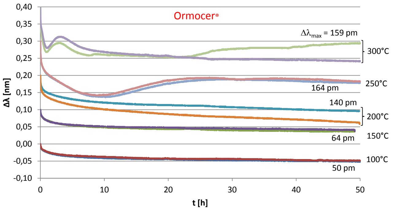
Figure 6: Wavelength stability (Bragg wavelength shift as a function of time) at different elevated temperatures for Ormocer® coated DTGs. \Delta\lambda_{\max} is the maximum wavelength shift from \Delta\lambda at t = 0 hours.
