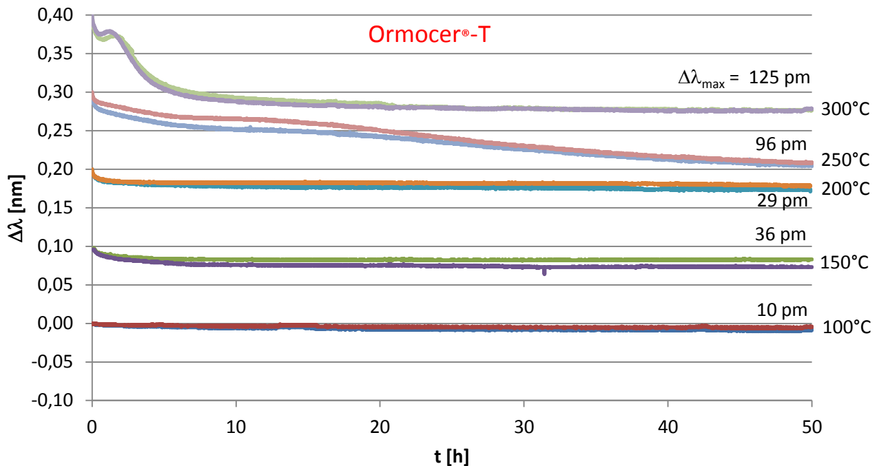
Figure 7: Wavelength stability (Bragg wavelength shift as a function of time) at different elevated temperatures for Ormocer®-T coated DTGs. \Delta\lambda_{\max} is the maximum wavelength shift from \Delta\lambda at t = 0 hours.
