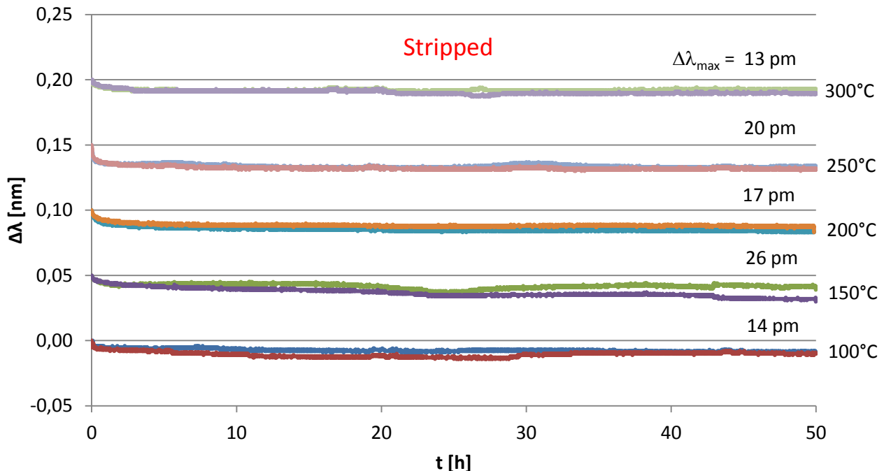
Figure 5: Wavelength stability (Bragg wavelength shift as a function of time) at different elevated temperatures for DTGs without coating (stripped). \Delta\lambda_{\max} is the maximum wavelength shift from \Delta\lambda at t = 0 hours.
