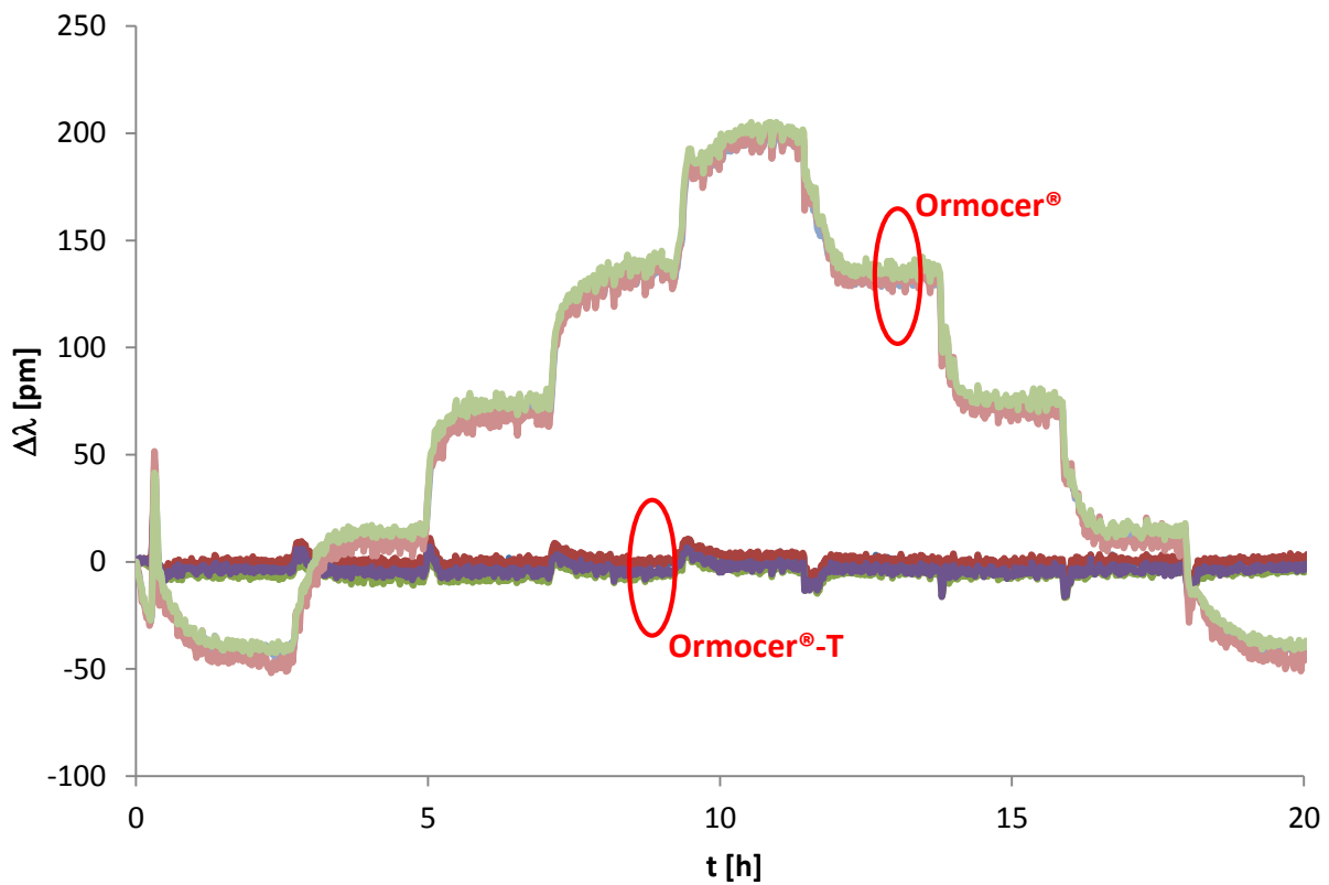
Figure 3: Measured wavelength shifts ( \Delta\lambda ) for both coating types as a function of time (t) during the RH calibration.
